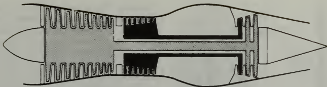
FIGURE 1-59. Dual-rotor turbine for split-spool compressor.
